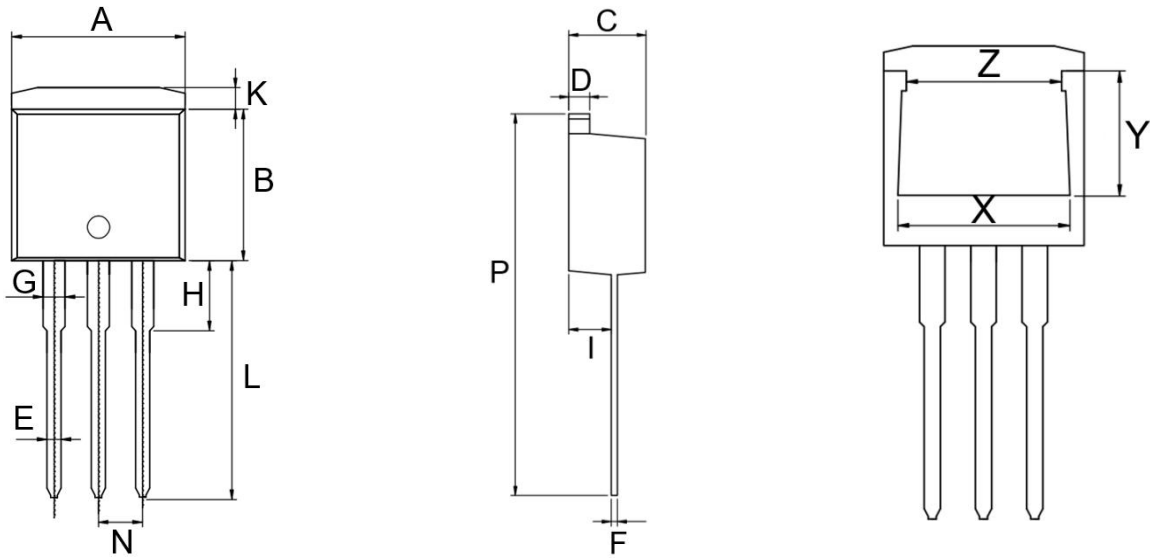
TO-262 Package
