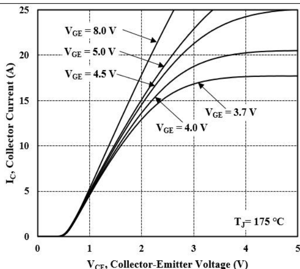
Figure 12 Collector-Emitter Voltage vs Collector Current
