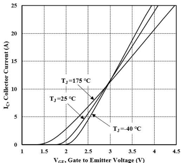
Figure 13 Transfer Characteristics
