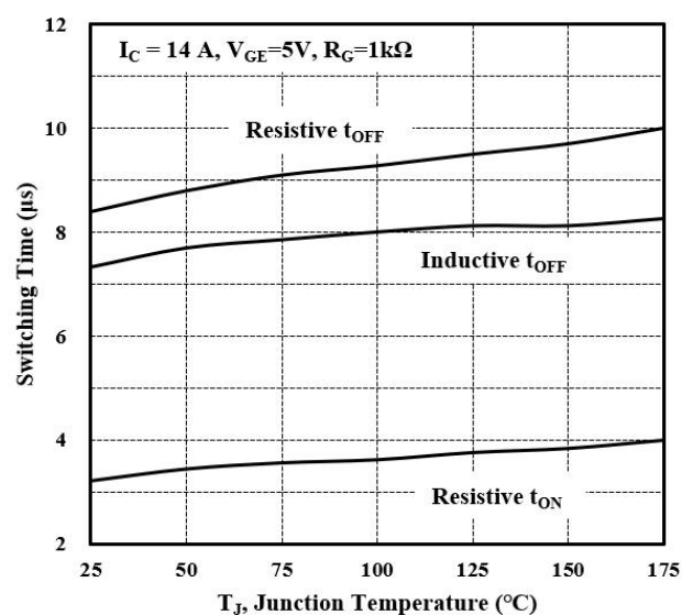
Figure 16 Switching Time vs Junction Temperature
