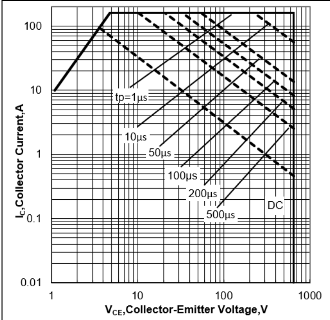
Figure 1. Forward Bias Safe Operating Area for TO247/TO3PF/TO3PN
