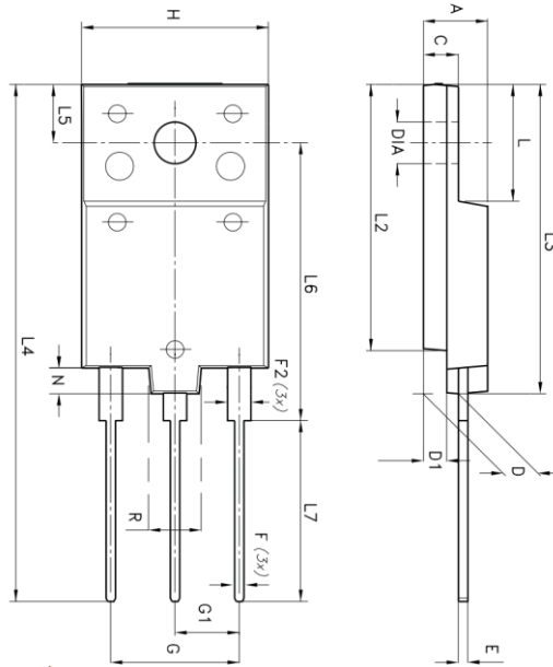
TO-3PF Package
