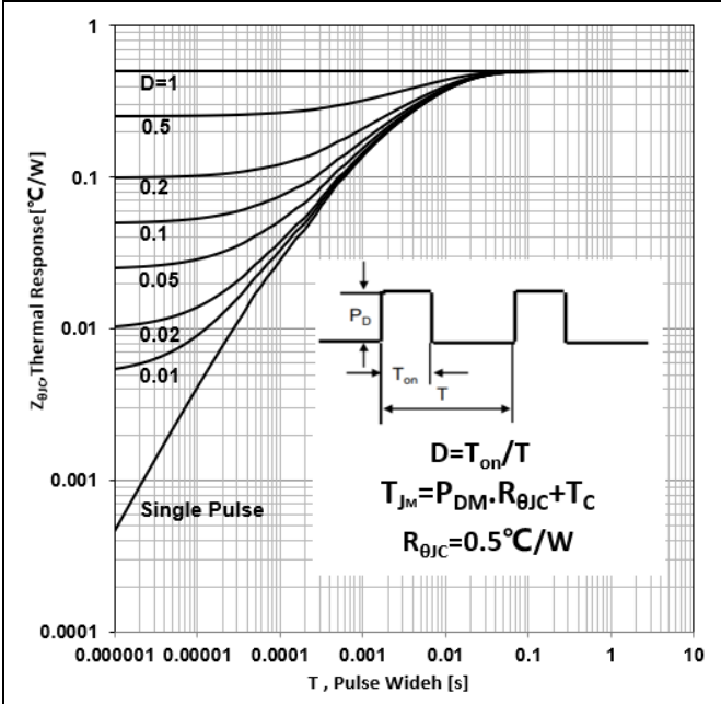
Figure 19. IGBT Transient Thermal Impedance vs Pulse Width(TO247/TO3PF/TO3PN)
