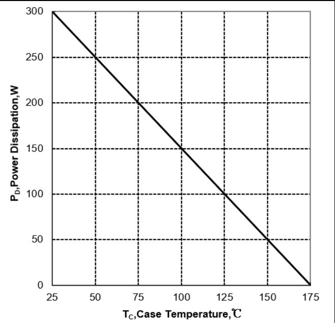
Figure 2. Power Dissipation vs Case Temperature for TO247/TO3PF/TO3PN
