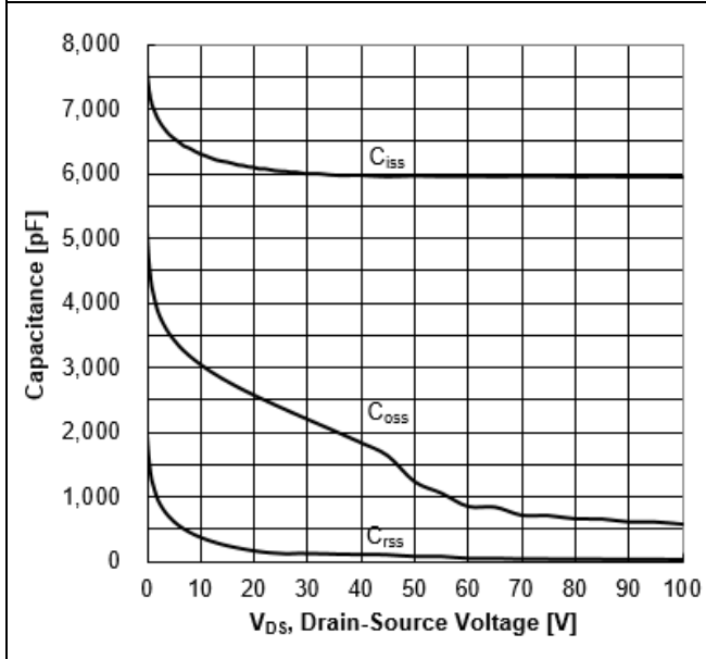
Figure 12. Capacitance Characteristics
